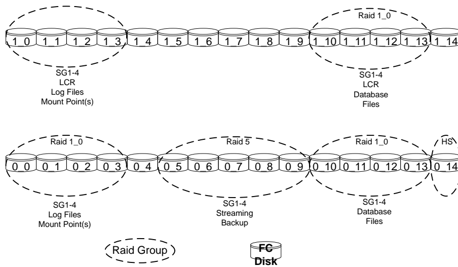
Figure 1 Building block layout
