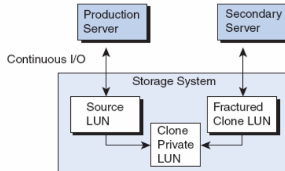
Figure 2. Clone example
