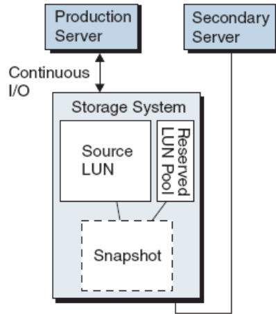
Figure 1. Snapshot example
